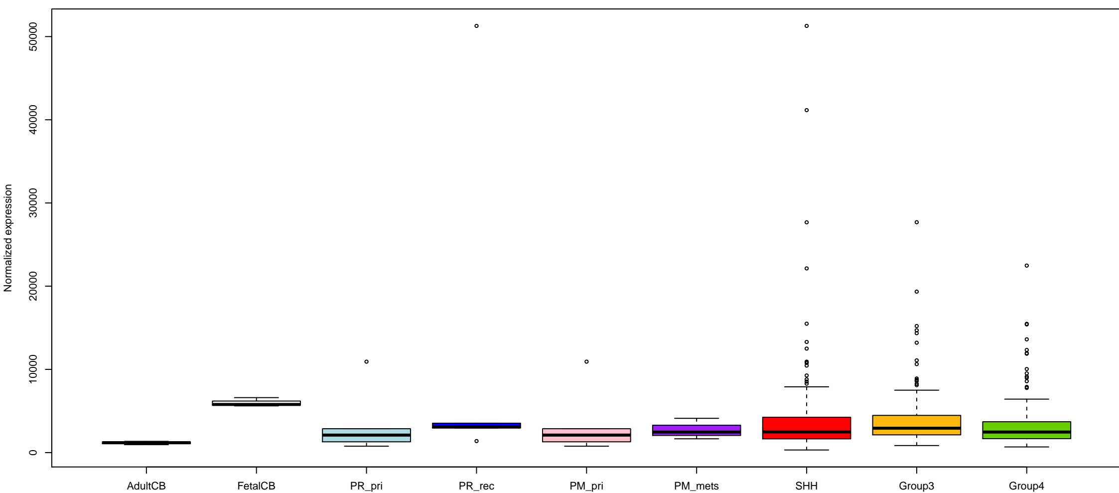
JAG1 expression (with outliers)
