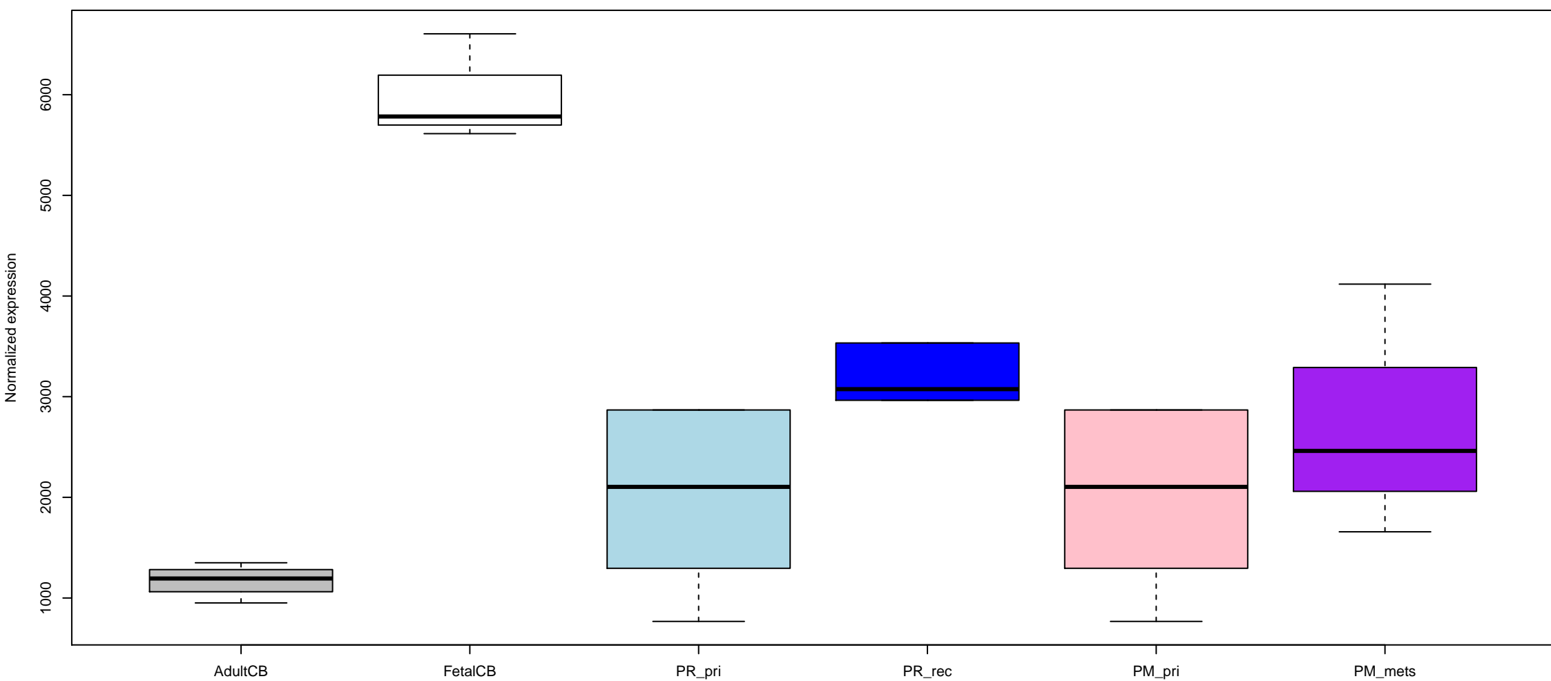
JAG1 expression (no outliers)
