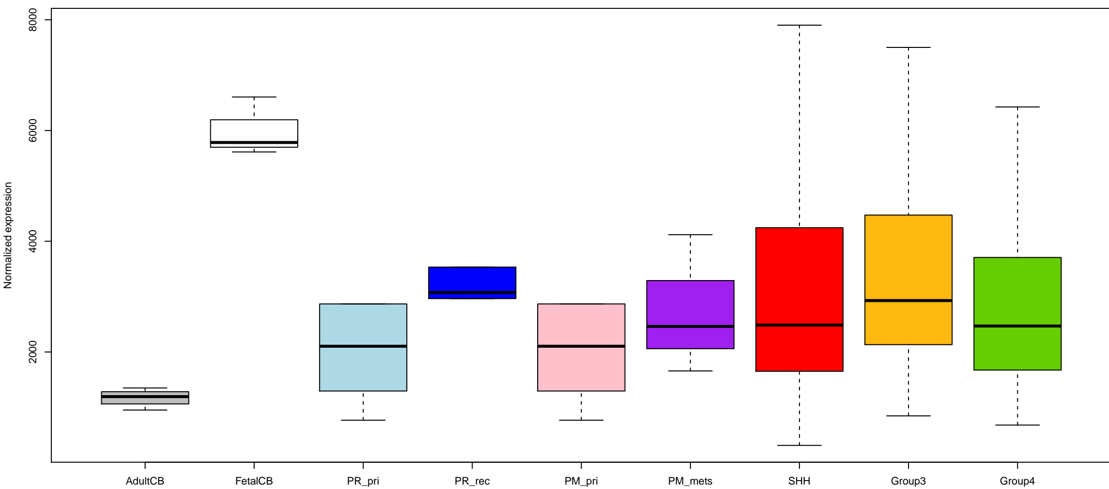
JAG1 expression (no outliers)
