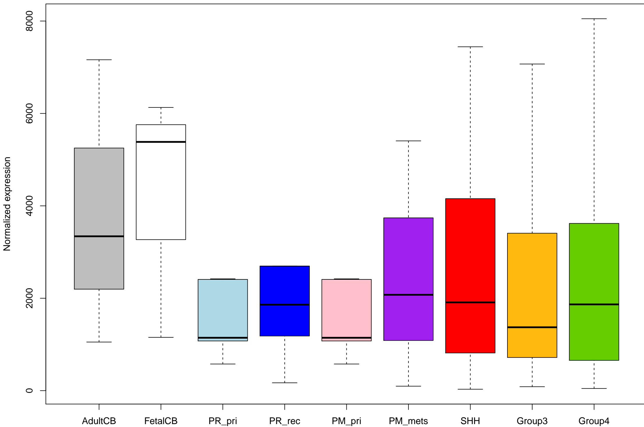
ENSG00000101463_TMEM90B_+ expression (no outliers)
