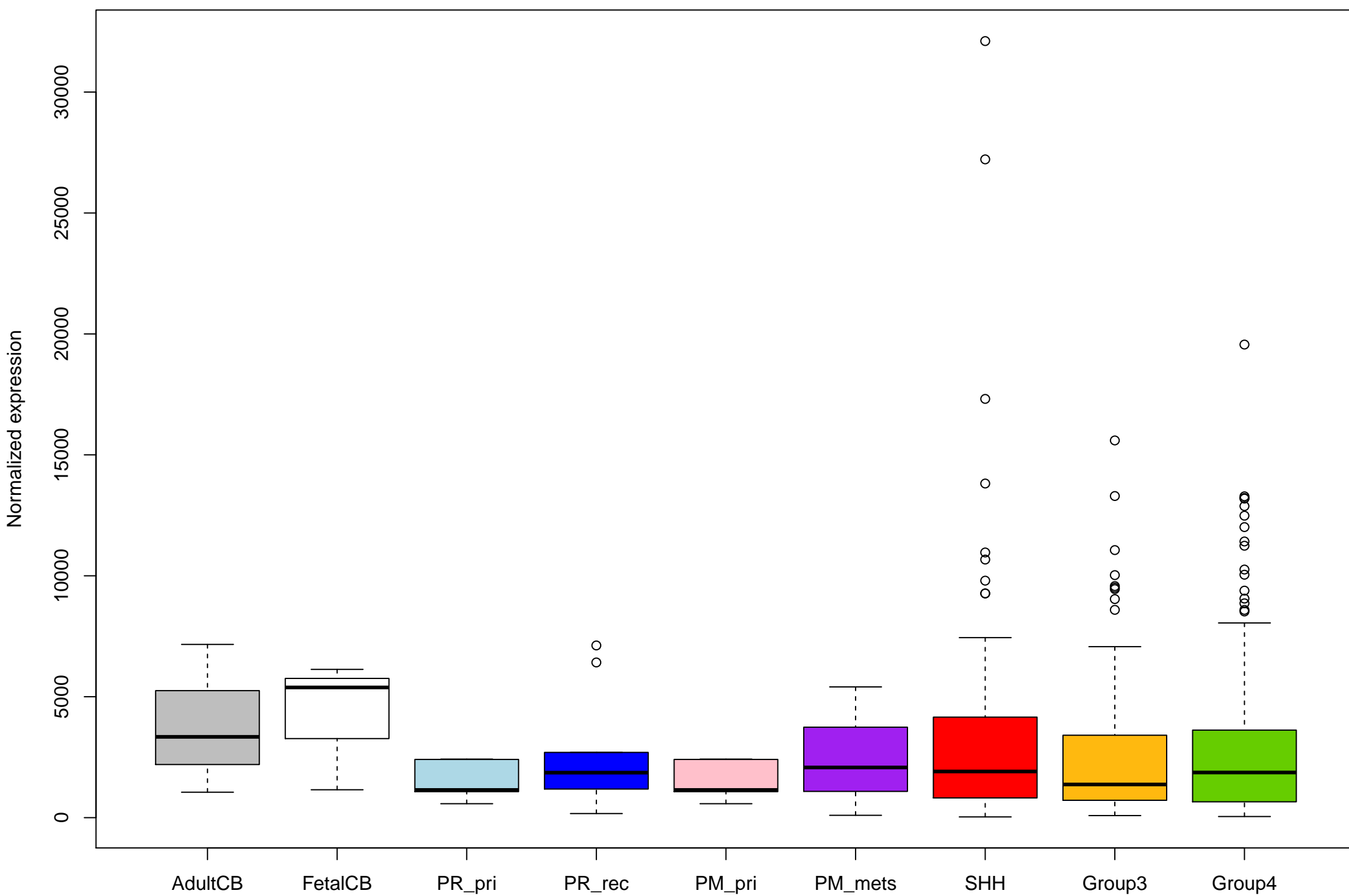
ENSG00000101463_TMEM90B_+ expression (with outliers)
