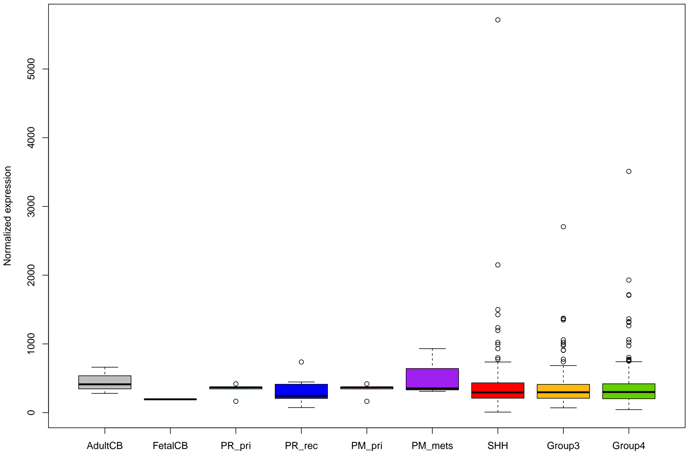
ENSG00000136867_SLC31A2_+ expression (with outliers)
