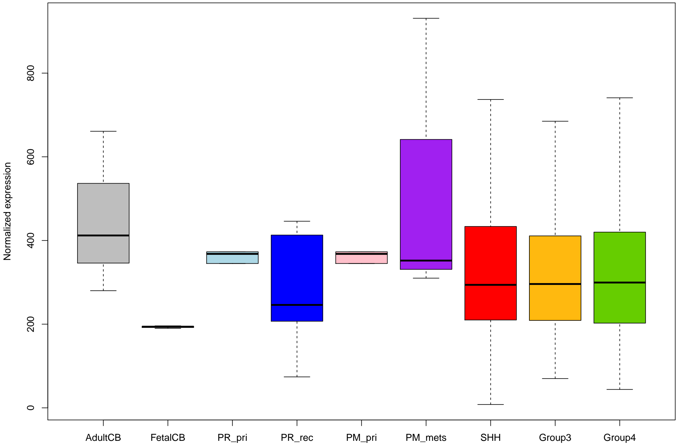
ENSG00000136867_SLC31A2_+ expression (no outliers)
