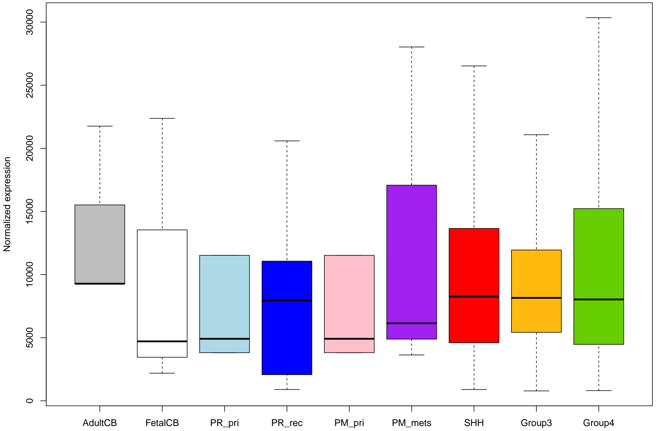
ENSG00000143153_ATP1B1_+ expression (no outliers)
