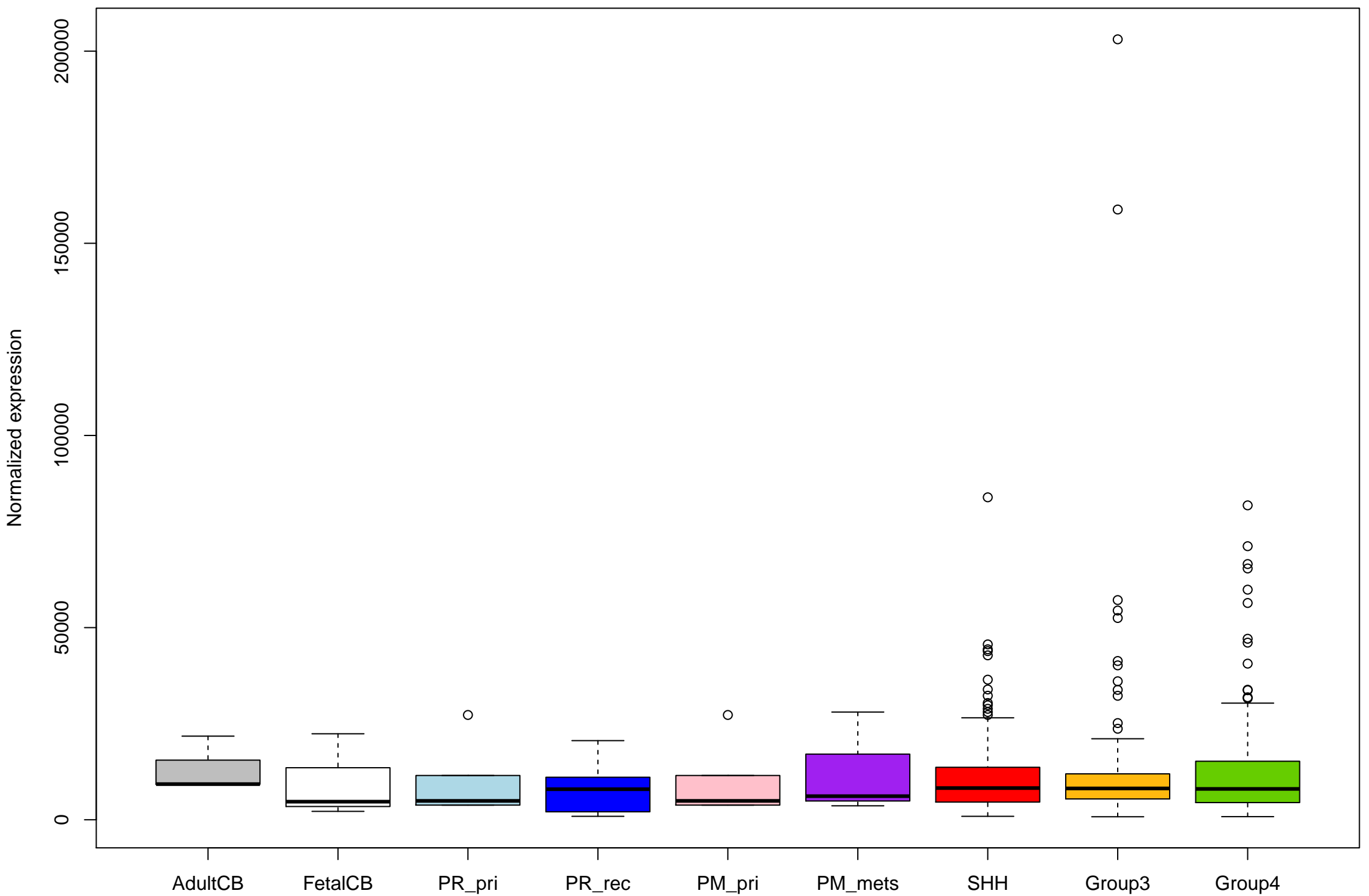
ENSG00000143153_ATP1B1_+ expression (with outliers)
