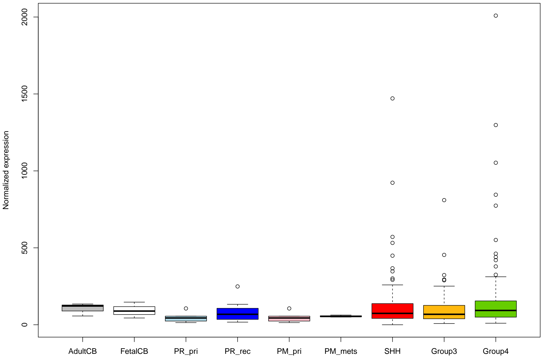
ENSG00000150637_CD226_ – expression (with outliers)
