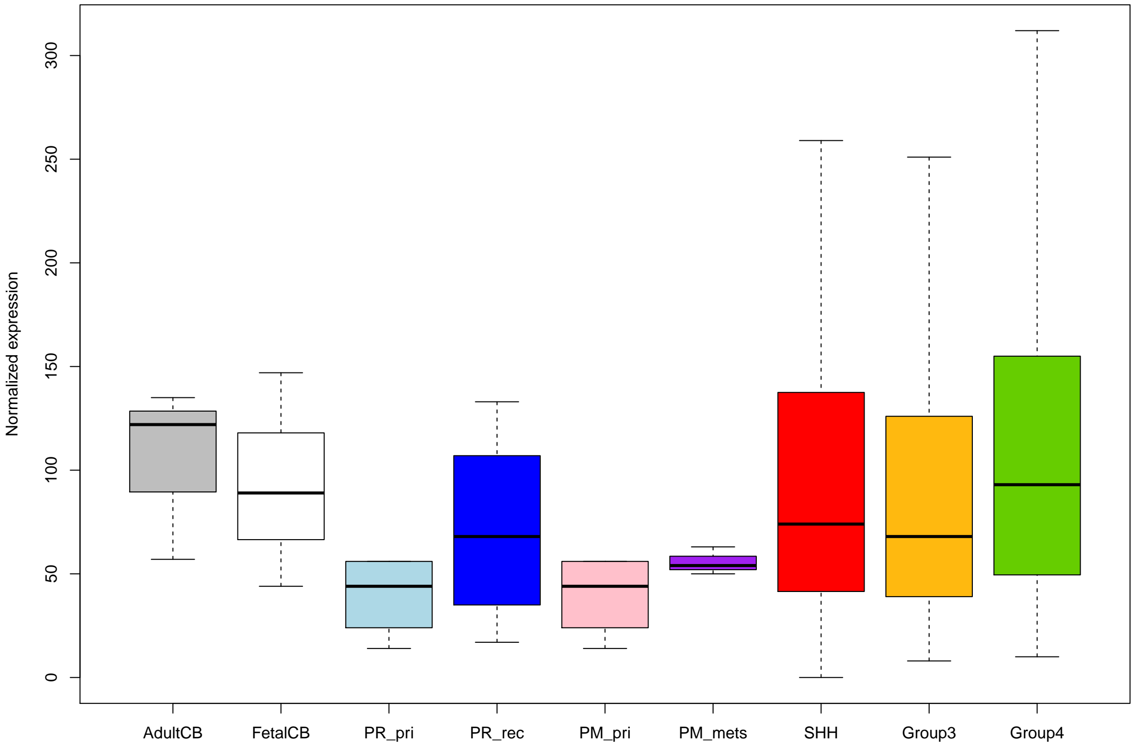
ENSG00000150637_CD226_ – expression (no outliers)
