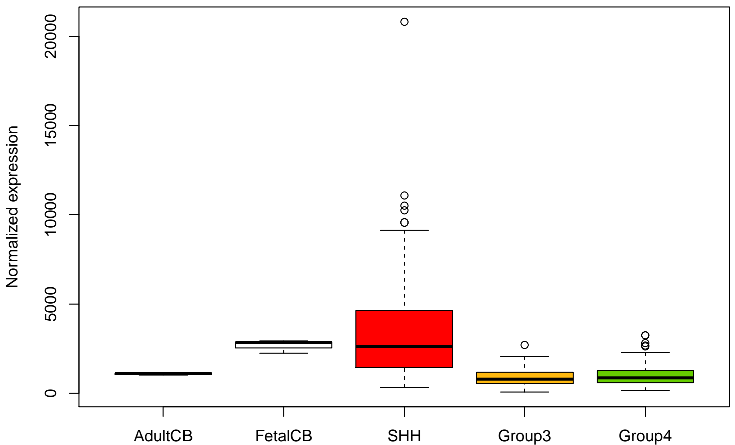
BCL2 ENSG00000171791 expression (including outliers)
