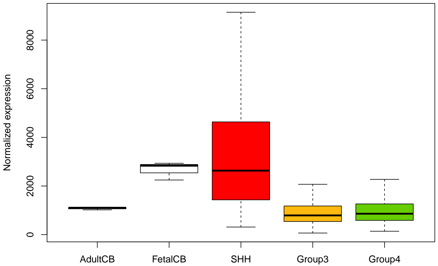
BCL2 ENSG00000171791 expression (no outliers)
