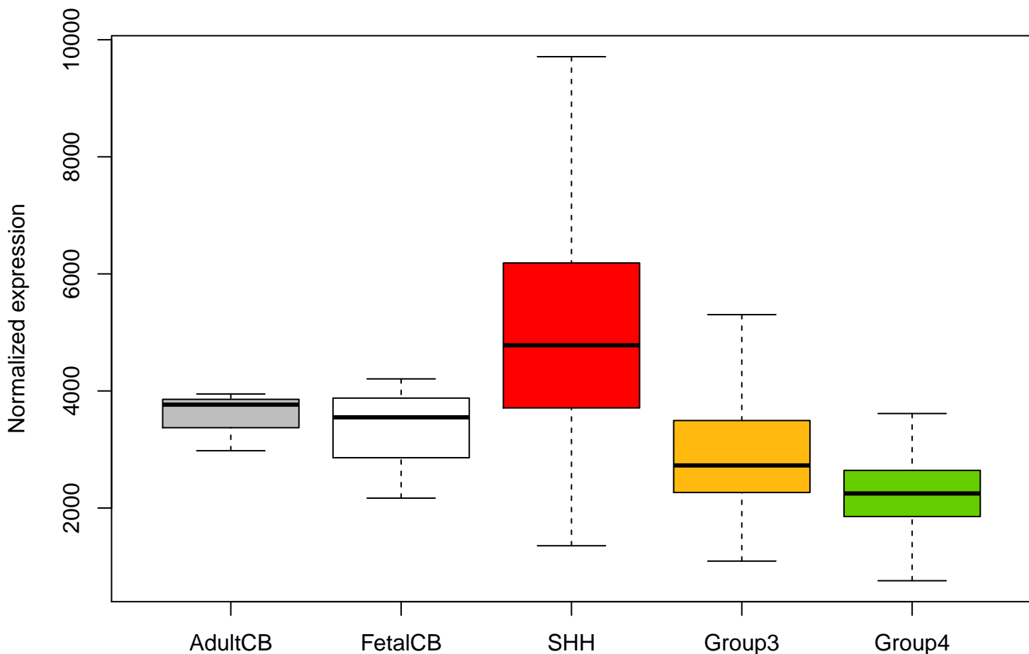
DRAM2 ENSG00000156171 expression (no outliers)
